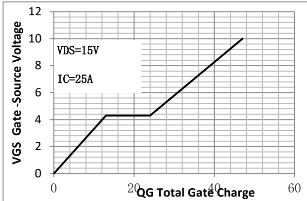
Fig.1 Gate-Charge Characteristics
