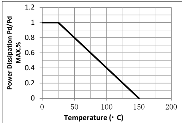
Fig.3 Power Dissipation
