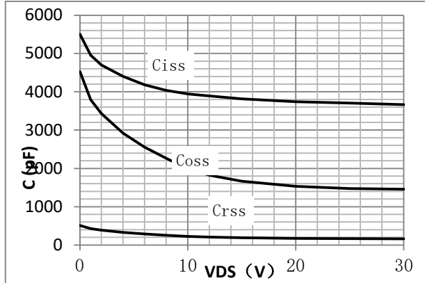
Fig.2 Capacitance Characteristics
